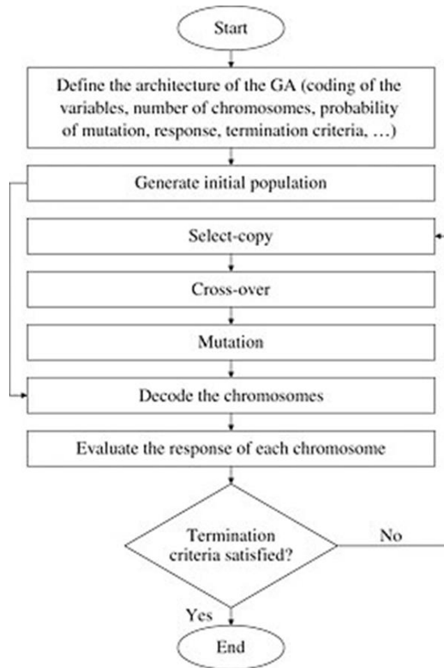
Figure 2: Flowchart of the optimization of the hybrid power system through Genetic Algorithm (Niazi & Leardi, 2012)
