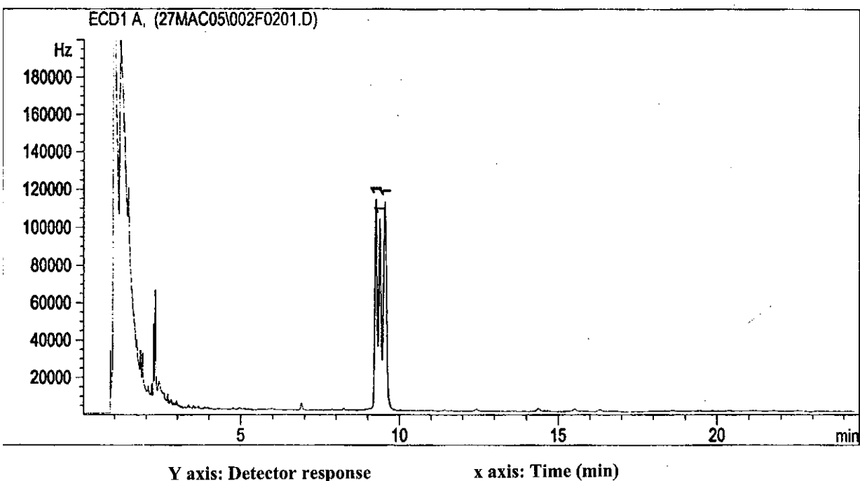
Figure 2c. Chromatograms for cypermethrin (1) fortified at 1 mg/kg for top soil of Tarat. First peak ( cis B), second peak ( trans C) and last peak ( cis B + trans D)
