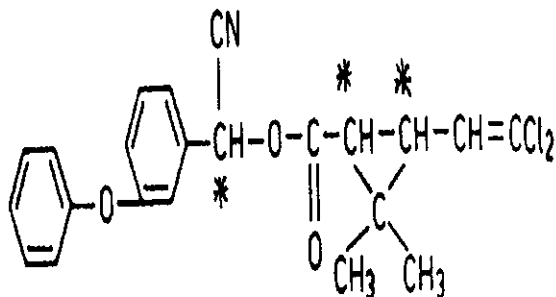
Figure 1. Chemical structure of cypermethrin. Asterisks denote asymmetric carbons. cis A = (1 R-cis-αR ; 1 S-cis-αS ), cis B = (1 R-cis-αS ; 1 S-cis-αR ), trans C = (1 R-trans-αR ; 1 S-trans-αS ) and trans D (1 R-trans-αS ; 1 S-trans-αR )
